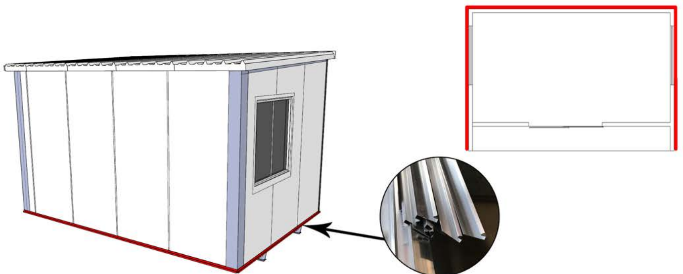
Step19 Installing starting part
